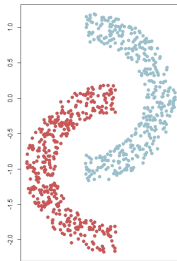
(g) Clustering
