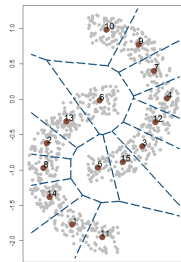
(c) Voronoi Cells
