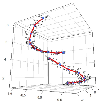
Skeleton Linear Spline
